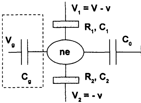
Fig.1. Charge-quantized double-barrier structure. Junctions with tunnel resistances R_{1,2} and capacitances C_{1,2} are shown as boxes. The self-capacitance C_0 of the central island is shown as a capacitor connected to a point with zero potential. The gate with capacitive coupling C_g may be absent from the system
