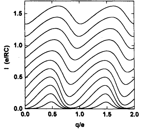
Fig.2. Single-electron transistor effect. Current I , defined by Eq. (4), versus the partial polarization q , defined by Eq. (8), at different transport voltages VC/e , starting at 0.2 at the bottom with increments of 0.2. k_B T = 0.05 e/C , C_1 = 0.7 C , C_2 = 0.1 C , R_2/R_1 = 10 , R = R_1 + R_2
