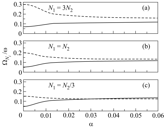
Fig.2. Critical velocities of outer condensate \Omega_{N_1}/\omega and the inner condensate \Omega_{N_2}/\omega as functions of \alpha for different values of N_2/N_1 . Dashed lines correspond to \Omega_{N_2}/\omega and solid lines – to \Omega_{N_1}/\omega
