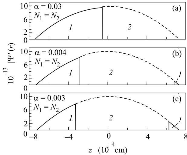
Fig.1. Density profiles of the condensates as functions of the vertical coordinate z for N_1 = N_2 . Figure (a) corresponds to \alpha > \alpha_c and figures (b), (c) – to \alpha < \alpha_c . Solid lines correspond to the |1\rangle atoms and dashed lines – to the |2\rangle atoms
