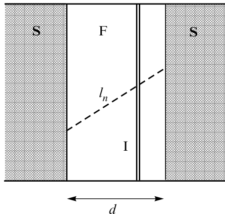
Fig.1. Junction configuration. The current flows from one superconductor (S) to the other through the ferromagnetic (F) layer (width d ) which a scattering region denoted by I. The exchange field is supposed to be parallel to the SF boundaries
