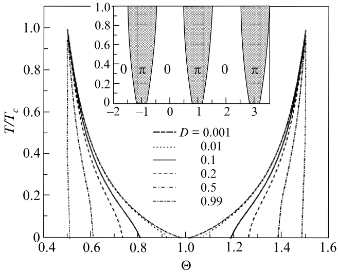
Fig.2. The temperature of the \pi - 0 transition at zero current versus the dimensionless exchange field \Theta = 2E_{ex}d/\pi\hbar v_F at different values of junction transparencies D . Only trajectories with l = 1 are taken into account which is justified if either one channel or many channels are present. Inset: phase diagram of the junction at D = 0.1 . The gray regions correspond to the \pi -phase, the white regions to the 0-phase
