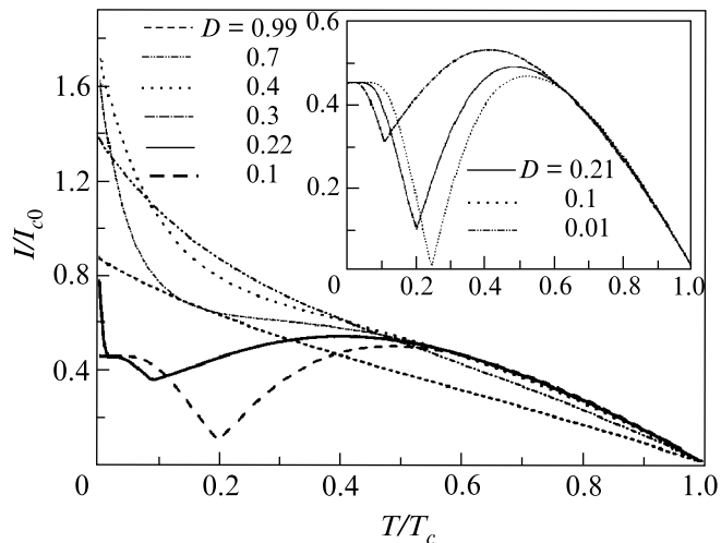
Fig.3. Dependence of the critical current on temperature for \Theta = 0.7 at different transparencies D . Cusps in the I_c(T) curves indicate the \pi - 0 transition. I_c is always nonzero at the cusp, see the inset. The plot of the critical current for D = 0.22 has two cusps. At low temperature and I \lesssim I_c , the junction with D = 0.22 is in the \pi -state, at intermediate temperatures (between two cusps) – in the 0-state, and for temperatures near T_c – again in \pi -state
