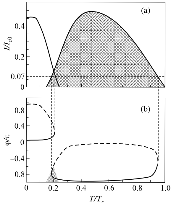
Fig.4. (a) The phase diagram of the junction for D = 0.1 , \Theta = 0.7 . The light gray region corresponds to the \pi -phase, the white to the 0-phase. The Gibbs potential has two minima of \varphi in [-\pi, \pi] in the dark gray region. The critical current (solid thick line) is the upper boundary of the phase diagram. (b) Temperature dependence of the phases corresponding to the d.c. current I = 0.07I_{c0} (dashed line parallel to the temperature axes in (a)). The thick solid line represents the stable solution of the equation I = I(\varphi) (minimum of the Gibbs energy), the dashed curve exhibits the unstable solution (maximum of the Gibbs energy). The equilibrium transition temperature ( I = 0 ) corresponds to T/T_c = 0.2
