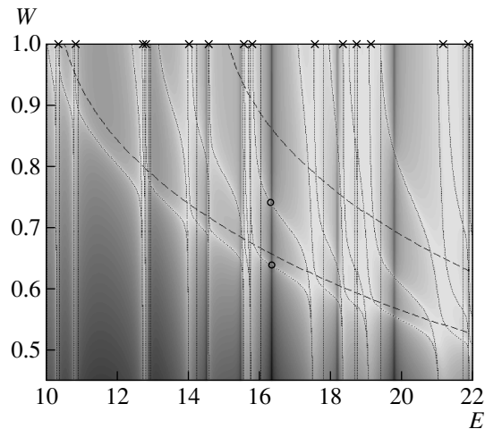
Fig.1. The probability \ln(T(E, W)) for the transmission through the double QD shown in Fig.3 versus energy and width of the wire. The eigenenergies of each single QD are marked by crosses. The eigenenergies of the wire are shown by dashed lines and those of the closed double QD system by thin dotted lines. In the present calculation, the eigenenergies of the closed system are almost the same as the eigenenergies of the open system. The radius of the QD in units of the width d of the input and output leads is 3d . The length of the wire is 2.5d . The size of all diaphragms is 0.6d
