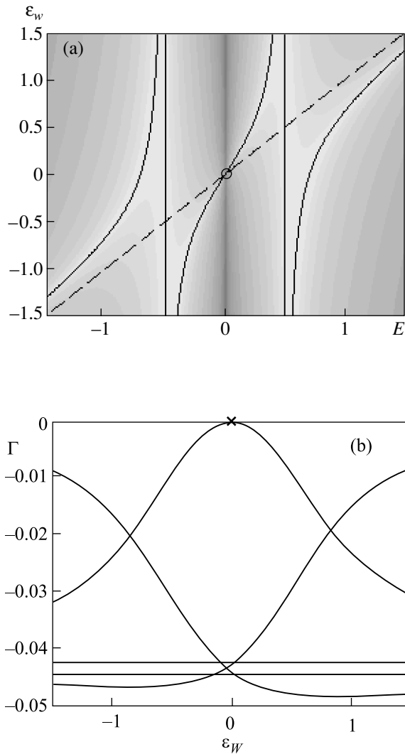
Fig.4. (a) The transmission through a system with two identical QDs that are connected by a wire, versus incident energy E and energy of the wire \varepsilon_w . The eigenenergies of (5) are shown by solid lines, and the energy \varepsilon_w of the wire is shown by the dashed line. The QDs have energies \varepsilon_{1,2} = \pm 1/2 . v = 1/2 , u = 1/4 . (b) The imaginary part of the 5 eigenvalues z_\lambda of the effective Hamiltonian (2) as a function of \varepsilon_w for E = 0.5 (at E = 0 , the widths of the two short-lived states are equal). One of imaginary parts is equal to zero at \varepsilon_w = \varepsilon_b = 0 for all energies E marked by cross
