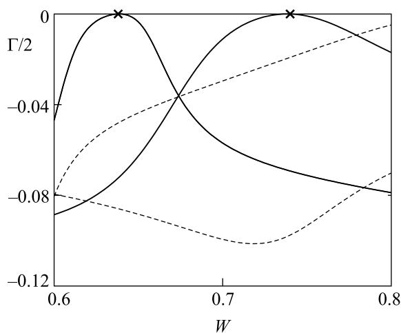
Fig.2. The imaginary part \Gamma_k of the first four eigenvalues z_\lambda as a function of W for E = 16.36 . The first two \Gamma_k which vanish at W = 0.638 and W = 0.74 are shown by the solid lines. Corresponding points are marked by crosses. They exactly correspond to points shown in Fig.1 by open circles
