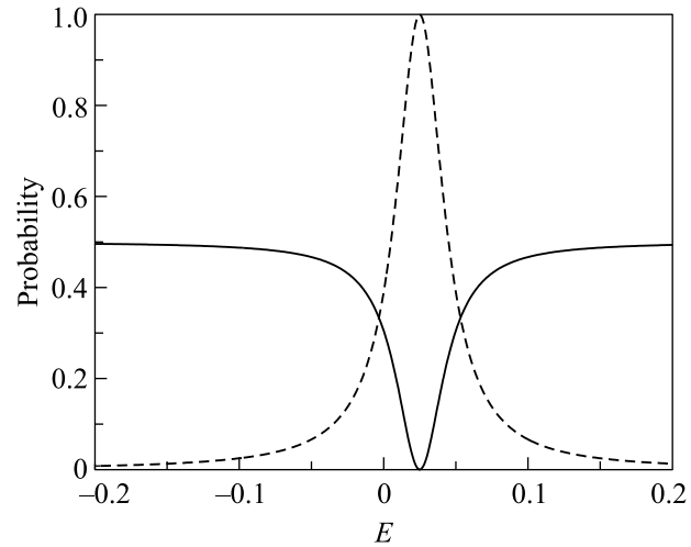
Fig.5. The probabilities for the electron to be in the wire (dashed line) and in the right and left QD (full line) as a function of the wire's energy. \varepsilon_{1,2} = \pm 1/2 , v = 1/2 , E = 0.02 , u = 0.2
