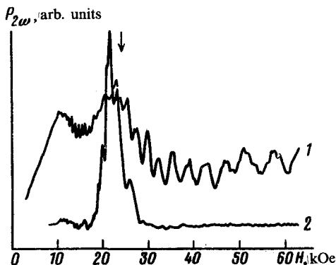
FIG. 3. Dependence of P_{2\omega} on H : 1) H_\omega \approx 6 Oe; P_{2\omega} = 0 dB. 2) H_\omega = 9 Oe; P_{2\omega} = 31 dB. The Bi sample is a cube; C_1 \parallel H; k_\omega \parallel C_2 ; T = 4.2 K.
