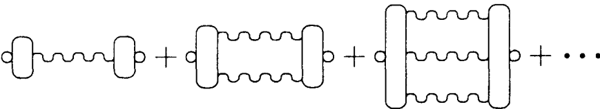
FIG. 2. The formally exact diagrammatic representation for K_{\epsilon\epsilon} , the first terms of an infinite series.
