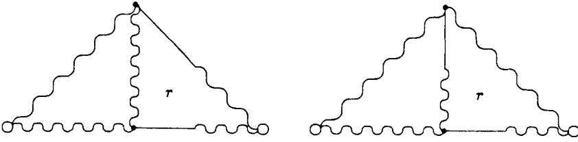
FIG. 1. The first diagrams for K_{\epsilon\epsilon} producing ultraviolet logarithms.
