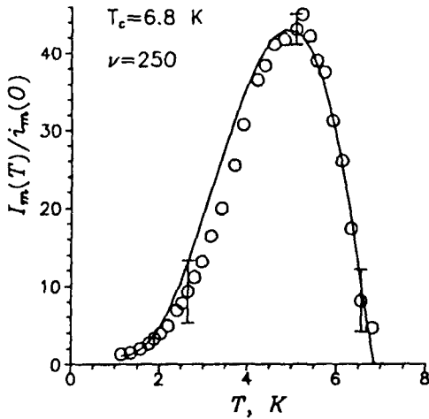
FIG. 2. Comparison of function (6) with experimental data from Ref. 4 on the alloy Zn_{41}Sb_{59} in a metastable state with an effective resistivity on the order of 10 \Omega \cdot \text{cm} .
