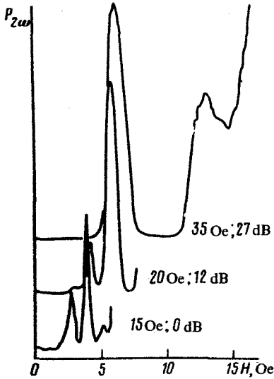
FIG. 2. The power P_{2\omega}(H) . The curves are labeled with H_{\omega} and with the relative sensitivity of the detection system.
