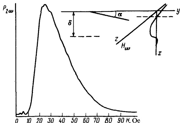
FIG. 1. The power P_{2\omega} versus H ; the amplitude of the exciting wave is H_{\omega} = 12 Oe.
