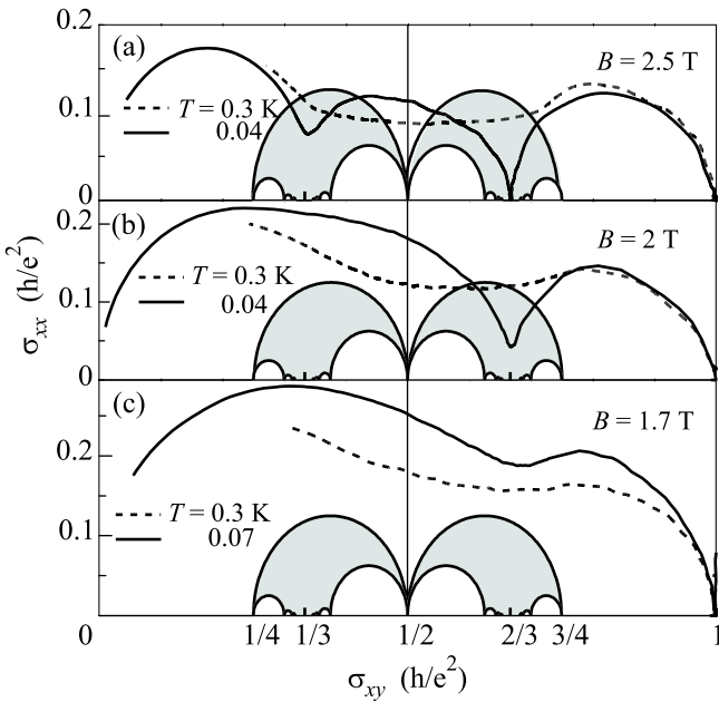
Fig.4. Magnetotransport data representation in the \sigma_{xy} - \sigma_{xx} plane for sample 1. Theoretical regions of conductivities converging to the 1/3- and 2/3- fractional QHE states when temperature goes to zero are shown by left and right grey areas, respectively. The dotted and solid lines present experimental conductivity traces obtained by sweeping gate voltage for T = 0.3 K and the base temperature, respectively. The traces in panels (a), (b), and (c) correspond to indicated magnetic fields
