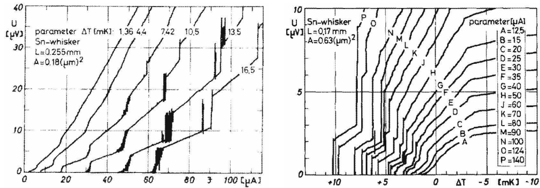
Fig. 1. Left panel: V-I characteristics of a tin whisker with length L and cross section A at various temperatures below the critical. Right panel: temperature dependencies of the voltage drop across the same sample at various fixed bias currents, indicated close to the curves. Adapted from J. D. Meyer et al. [3] https://doi.org/10.1016/0375-9601(72)90802-X . By courtesy of Elsevier
