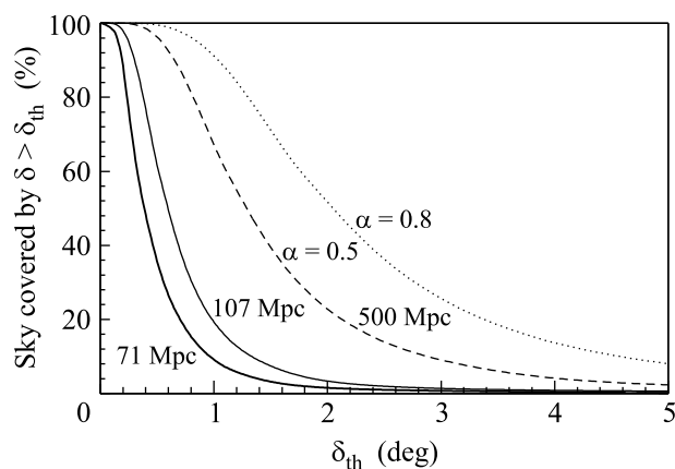
Fig.2. Cumulative fraction of the sky with deflection angle larger than \delta_{\text{th}} , for several values of propagation distance (solid lines). We also include an extrapolation to 500 Mpc, assuming self similarity with \alpha = 0.5 (dashed line) or \alpha = 0.8 (dotted line). The assumed UECR energy for all lines is 4.0 \cdot 10^{19} eV
