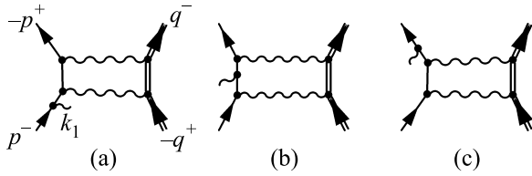
Fig.1. Set of box-type FD used in calculation
