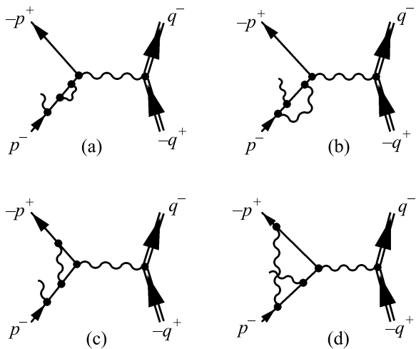
Fig.2. Set of vertex FD used in our calculation
