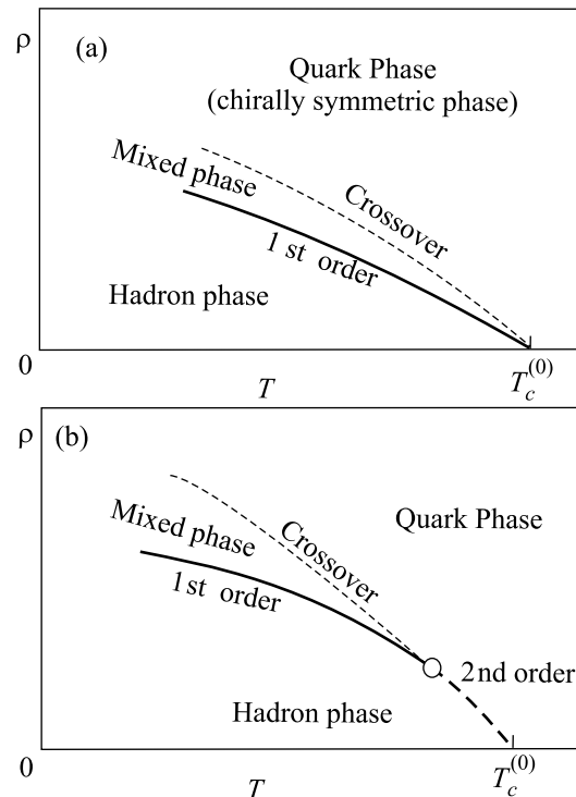
Fig.2. The qualitative phase diagram at finite baryon density and temperature based on the analysis (a) without and (b) with indication of the approximate 2 nd order transition domain
