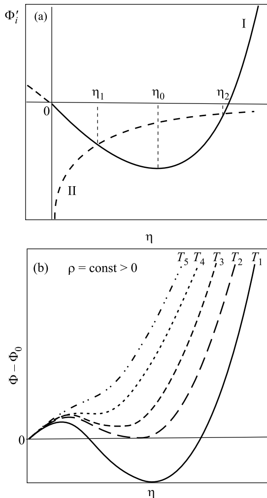
Fig.1. (a) Graphical representation of Eq. (4): I is the first term and II the second term (with the opposite sign) in the r.h.s. of the equation. (b) The thermodynamical potential (3) vs. the chiral condensate at a fixed baryon density \rho > 0 . At low enough temperatures, T = T_1 , the system resides in the chirally broken (hadron) phase. The first order phase transition to the quark phase takes place at T_{\text{ph}} = T_2 > T_1 . At somewhat higher temperatures, T_3 > T_{\text{ph}} the system is in a mixed state. The temperature T_4 \equiv T_{\text{cont}} corresponds to a continuous transition to the pure quark phase, in which the thermodynamical potential has the form T_5
