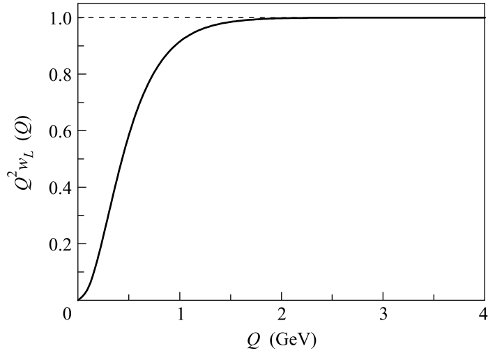
Fig.3. Normalized w_L invariant function in the singlet case (solid line) and nonsinglet case (dashed line)
