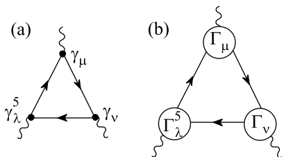
Fig.1. Diagrammatic representation of the triangle diagram in the local perturbative theory (a); and in the instanton model with dressed quark lines and full quark-current vertices (b)
