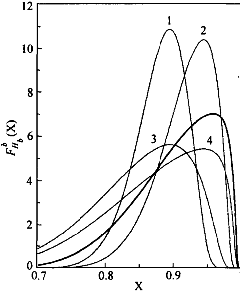
Fig.1. The distribution functions F_B^b(x) (solid line) and F_{\Lambda_b}^b(x) (thin lines) defined by Eq. (7) versus the LF momentum fraction x . Labels 1 to 4 on the curves refer to the cases \beta_{bu} = 0.3 GeV, m_{ud} = 600 MeV; \beta_{bu} = 0.3 GeV, m_{ud} = 300 MeV; \beta_{bu} = 0.6 GeV, m_{ud} = 600 MeV; \beta_{bu} = 0.6 GeV, m_{ud} = 300 MeV, respectively
