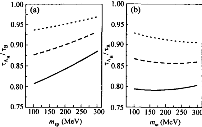
Fig.2. The lifetime ratios \tau_{\Lambda_b}/\tau_B for \beta = 0.3 GeV ( r = 0.3 ) (solid line), \beta = 0.45 GeV ( r = 1 ) (long-dashed line), and \beta = 0.6 GeV ( r = 2.37 ) (short-dashed line). (a) m_{ud} = m_u + m_d , and (b) m_{ud} \sim \frac{1}{2}(m_u + m_d - m_\pi)
