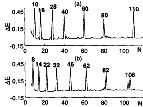
Fig.4. Magic numbers calculated at values of parameters as for Fig.2. The magic numbers corresponding to a pure quadrupole deformed harmonic oscillator are indicated in (a) for the ratio 1 : 2 : 2 and in (b) for the ratio 1 : 3 : 2
