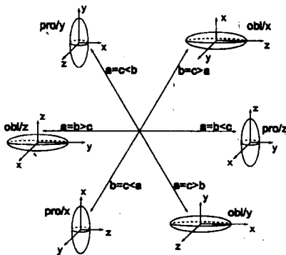
Fig.1. Shapes in the a, b, c plane. Spherical symmetry ( a = b = c ) is at the center while axially symmetric prolate and oblate shapes are obtained along the various axes. A genuine tri-axial quadrupole deformation ( a \neq b \neq c ) occurs between the axes
